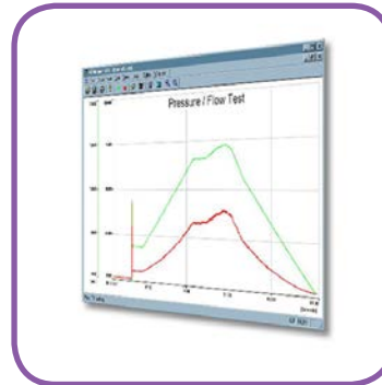
HPMcomm software
