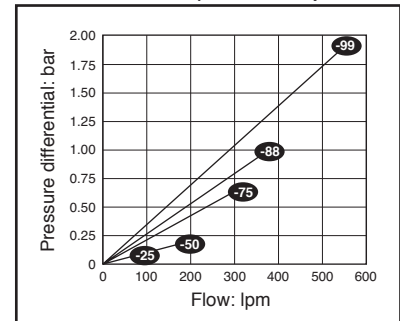
Series 5 (1 1/4" - 2")
